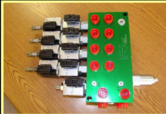
P.N. 87127 FOUR FUNCTION ELEC VALVE
